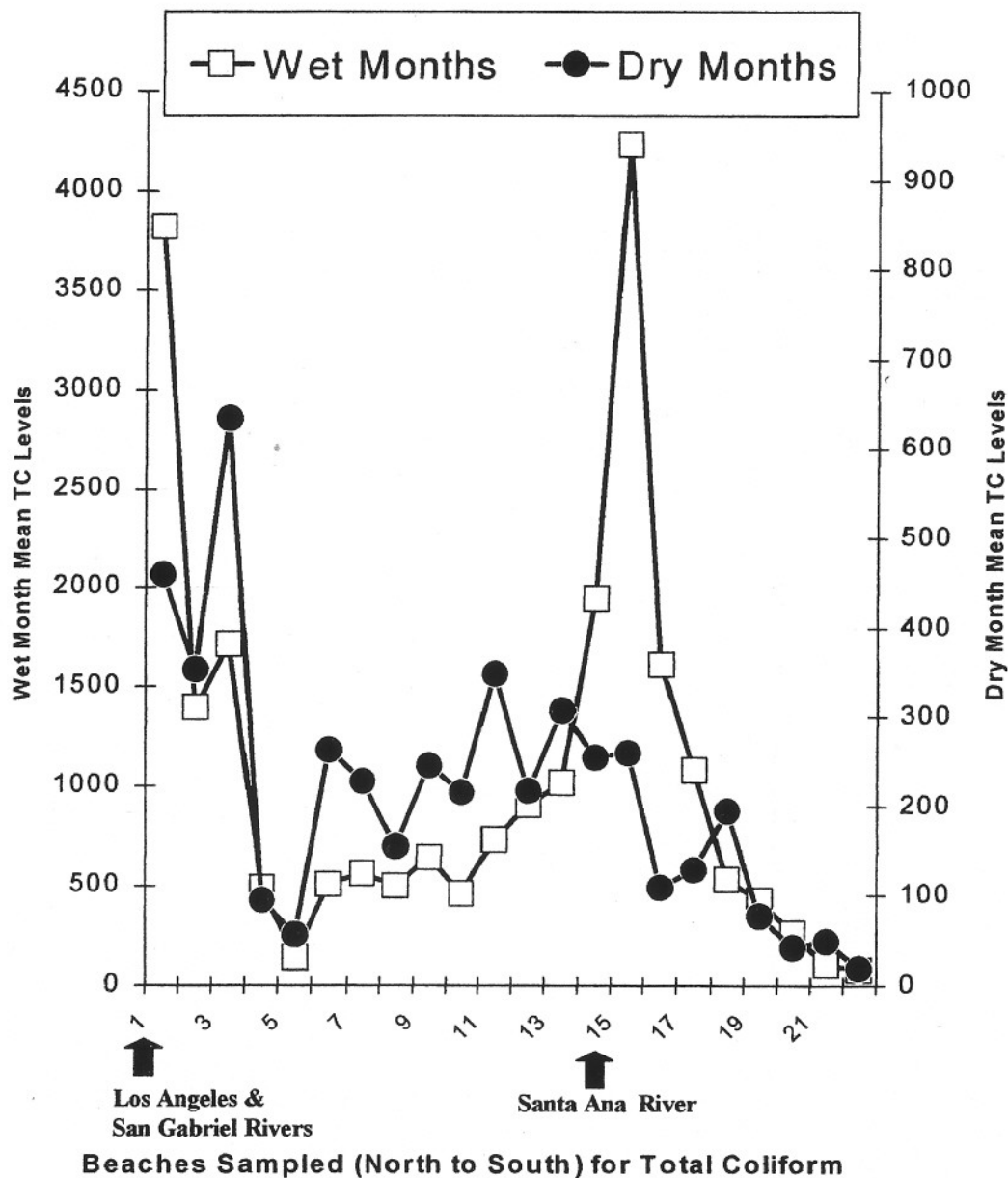
Figure 3—Mean total coliform levels (cfu) for 22 sampling stations by wet and dry months for January 1997 to July 1999. Wet month scale is 4.5 times the dry month scale. Source: Orange County Health Care Agency.
