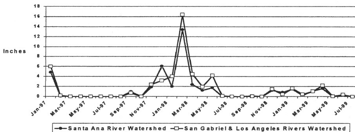
Figure 4—Mean precipitation per month for Santa Ana River watershed and combined San Gabriel and Los Angeles Rivers watersheds (in. × 25.4 = mm). Source: Western Regional Climate Center .
