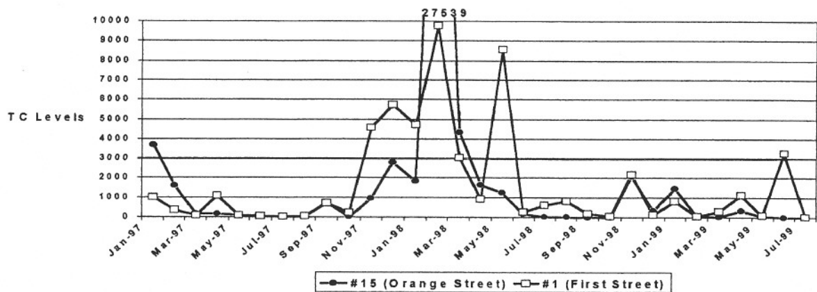
Figure 6—Mean total coliform levels per month at Rivermouth Beaches: station 15 (Orange Street) and station 1 (1st Street). Source: Orange County Health Care Agency.
