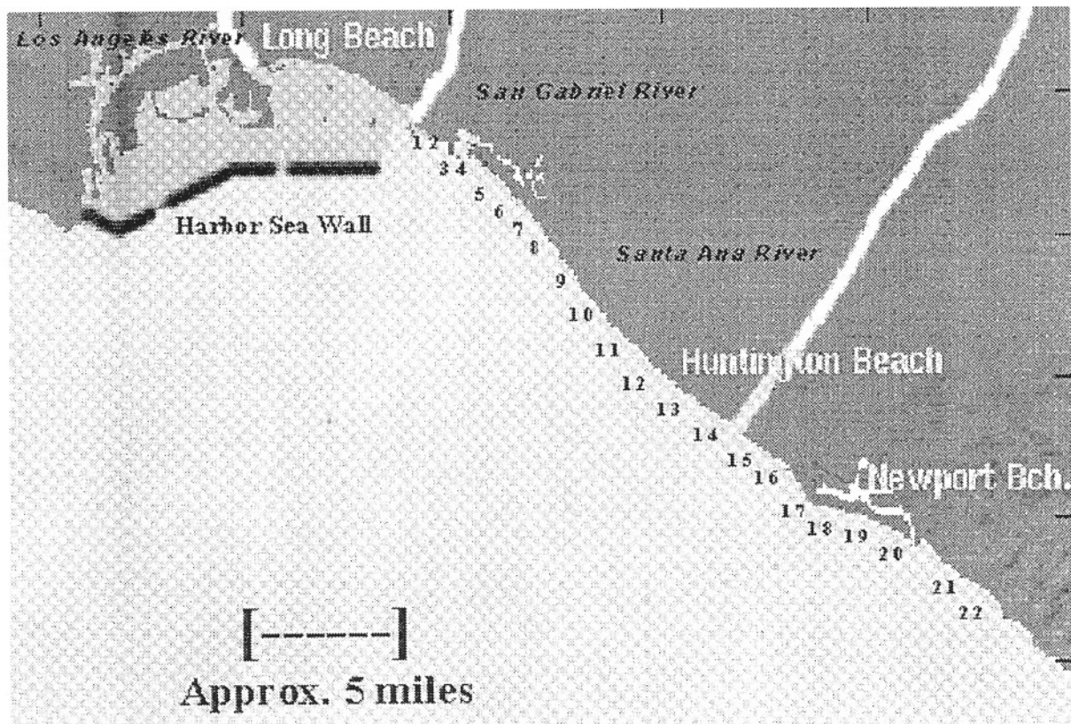
Figure 2 —Twenty-two monitoring stations along North Orange County's coastline (mile \times 1.609 = km). Source: University of California, San Diego.
