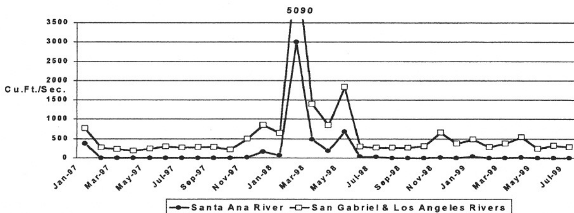
Figure 5—Mean discharge per month for Santa Ana and Combined San Gabriel and Los Angeles Rivers (cfs × 0.028 32 = m 3 /s). Source: U.S. Geological Service .
